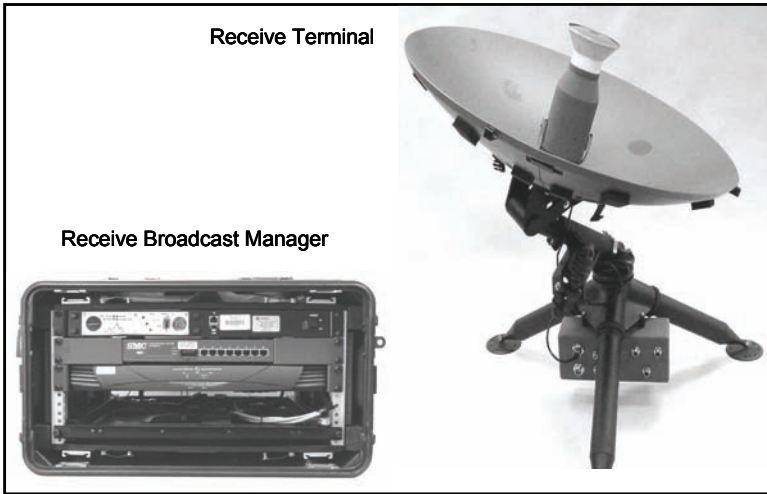
Figure 6-4. Transportable ground receive suite
